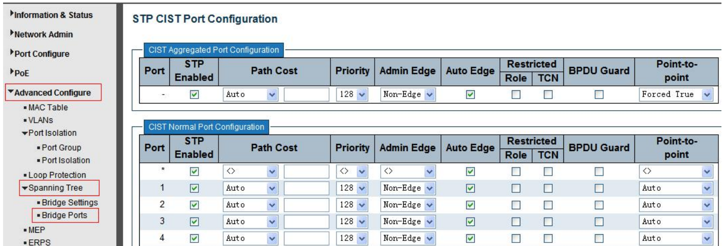
Figure 5-5 STPConfiguration Screen
