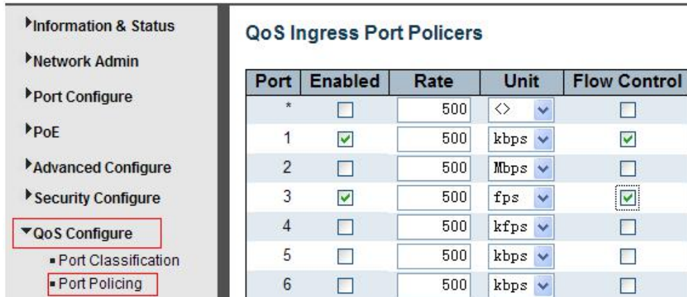
Figure 6-2Port PolicingConfiguration Screen
