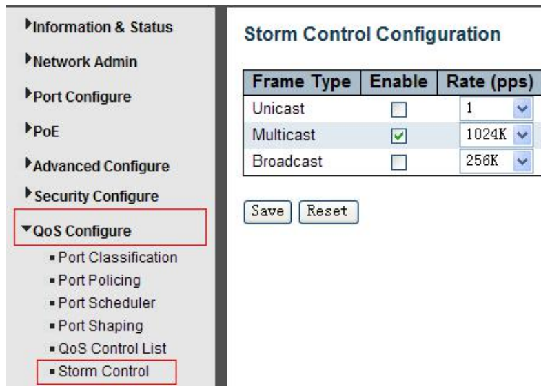
Figure 6-3Port PolicingConfiguration Screen
