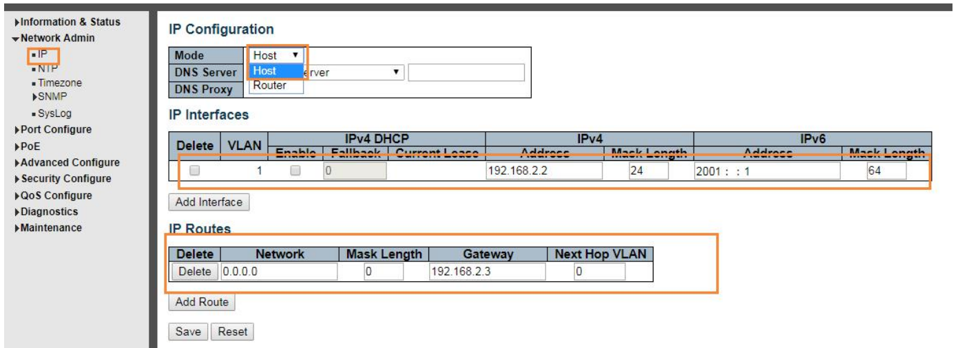
Figure 2-1IP Configuration Screen
