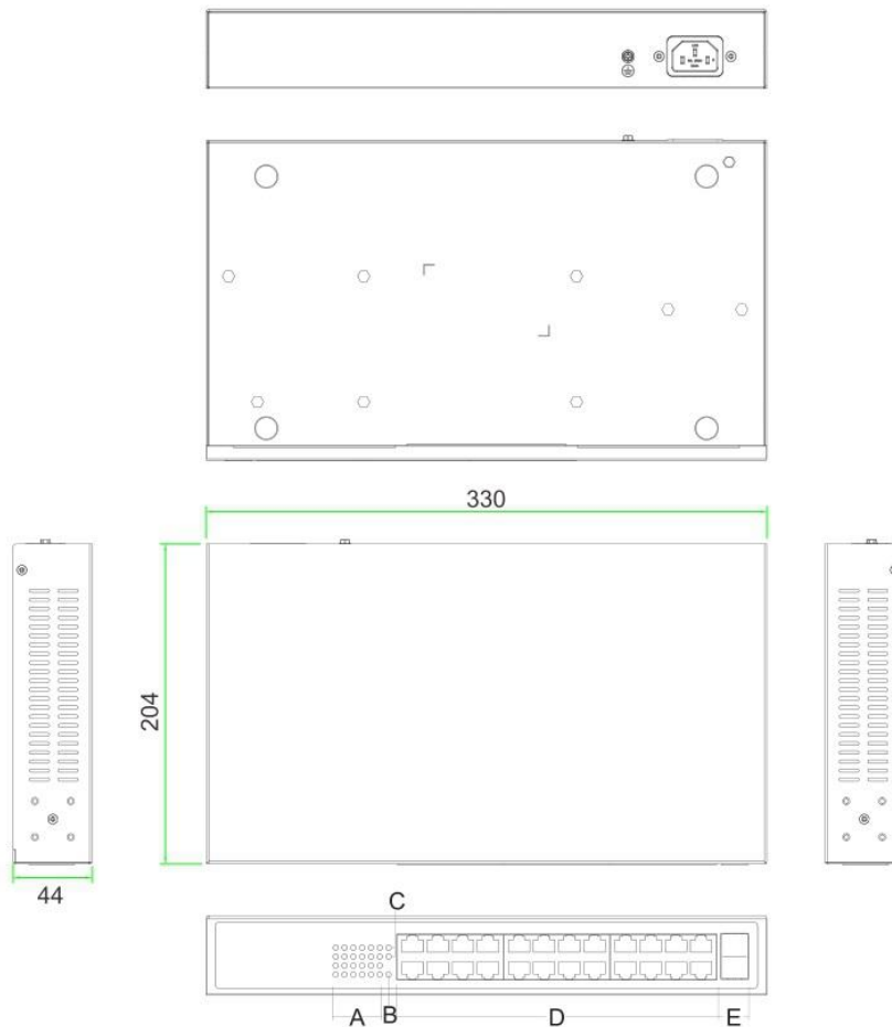
A. Work indicator for RJ45 port B. Power indicator C. Work indicator for SFP port D. 24* 10/100/1000M RJ45 ports E. 2*1000M uplink SFP ports
